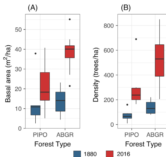
Fig. 3. Boxplots showing (A) basal area and (B) forest density in reconstruction plots in 1880 and 2016. The lower and upper hinges of boxplots correspond to the first and third quartiles of basal area and forest density observations within plots within each forest type. The black line dividing the box represents the median observation. There was a statistically significant difference between historical forest density in PIPO and ABGR stands. There was no significant difference in historical basal area between forest types. There is a statistically significant difference between contemporary PIPO and ABGR plot basal area and density. Note that there is a greater difference between contemporary ABGR and PIPO stands than there was historically.
